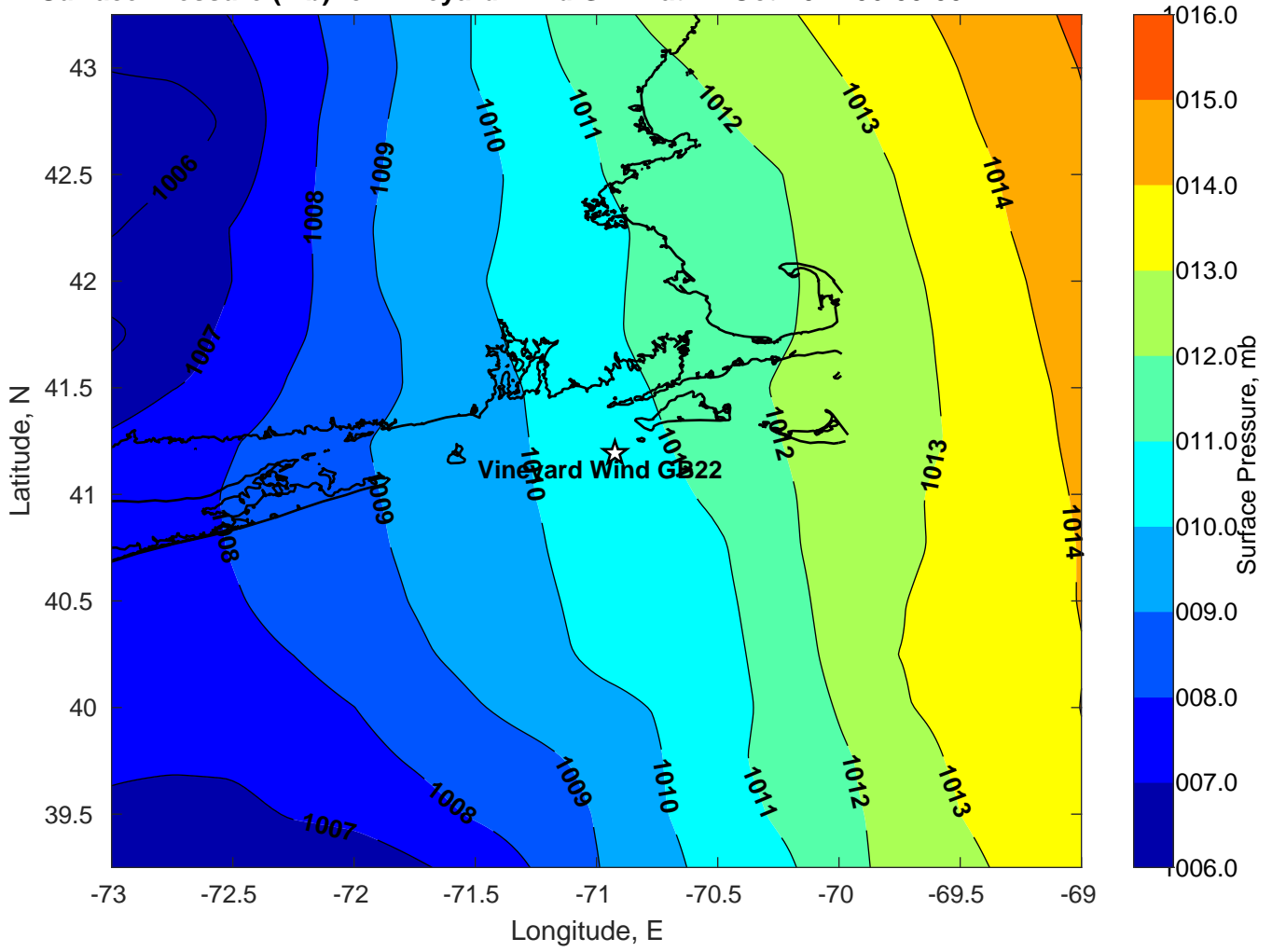
Surface Pressure (mb) for Vineyard Wind GB22 at 14-Oct-2022 06:00:00
